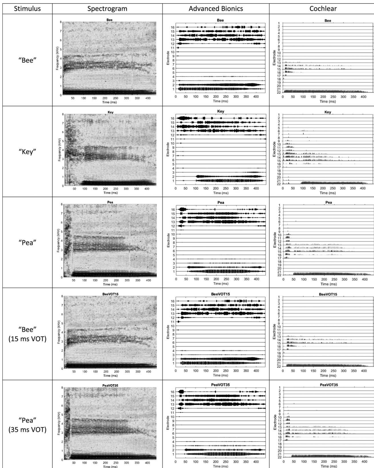
FIG. 3. Spectrograms of the five word tokens used in this study (second column). Simulated electrodegrams showing pulsatile stimulation patterns for the HiResolution F120 Sequential (HiRes F120S) processing strategy from Advanced Bionics (third column) and the advanced combinational encoder (ACE) processing strategy from Cochlear (fourth column). All electrodegrams were simulated using standard clinical maps. Electrode arrangement in the electrodegrams was based on ascending frequency from bottom to top of graph instead of the order of electrode numbers.
