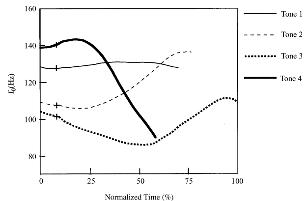
Figure 1. Mean F 0 contour of four Mandarin tones in the /ma/ monosyllable produced in isolation. The time course is normalized, with all tones plotted with their average duration proportional to the average duration of T3 (Xu, 1997, p. 67, reprinted with permission).
