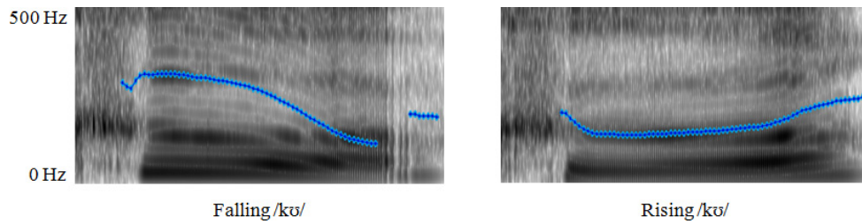
Figure 2. Spectrogram and pitch contour of falling /ku/ (left) and rising /ku/ (right).
